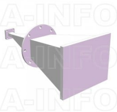
LB-34-25-A2SPO Standard Gain Horn Antenna 22-33GHz 25dB Gain Rectangular Waveguide Interface
